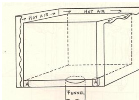
FIGURE 2. DRYING STOVE WITH THE FRONT WALL AND LID REMOVED SHOWING INTERIOR OVEN SUPPORTED BY BLOCKS (A).
